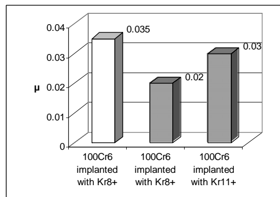
Fig. 5: Friction coefficient \mu - steel 100Cr 6, F=10N .
