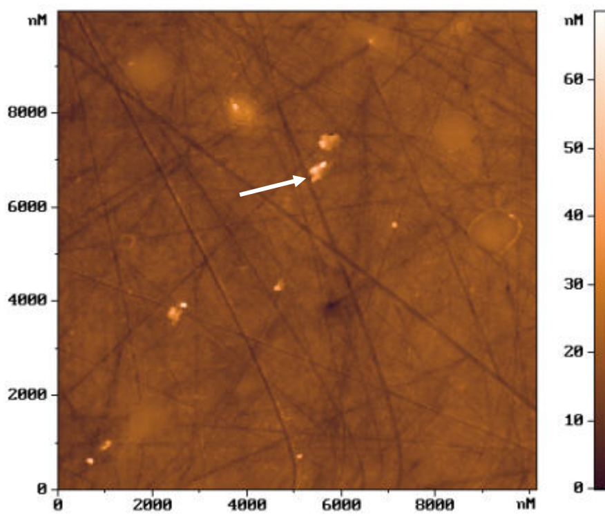
Fig 8: AFM 2D image of the same sample
