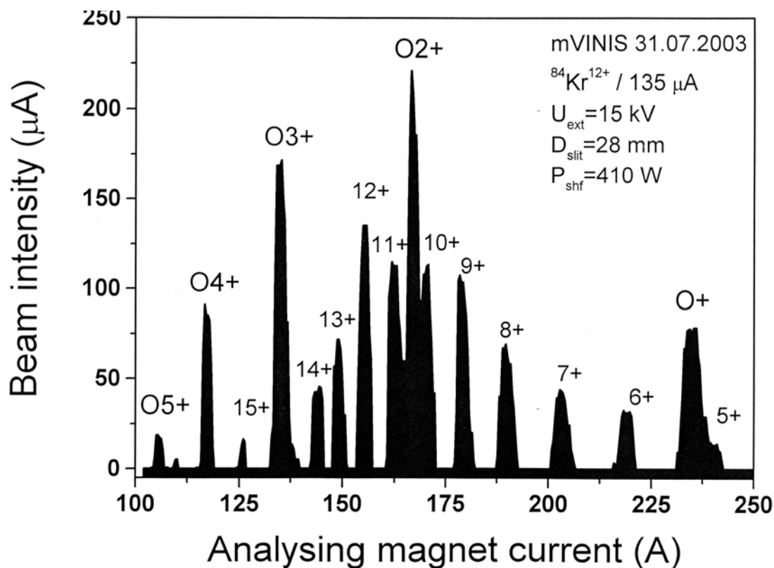
Fig 2: Krypton spectrum
