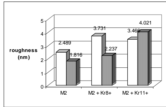
Fig 4: AFM surface roughness – M2 steel
