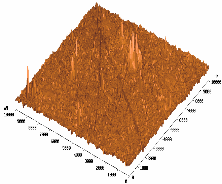
Fig.7: AFM image of surface roughness – M2 steel after Kr 8 + implantation.
