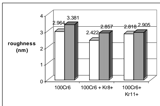
Fig 3: AFM surface roughness – 100Cr 6 steel
