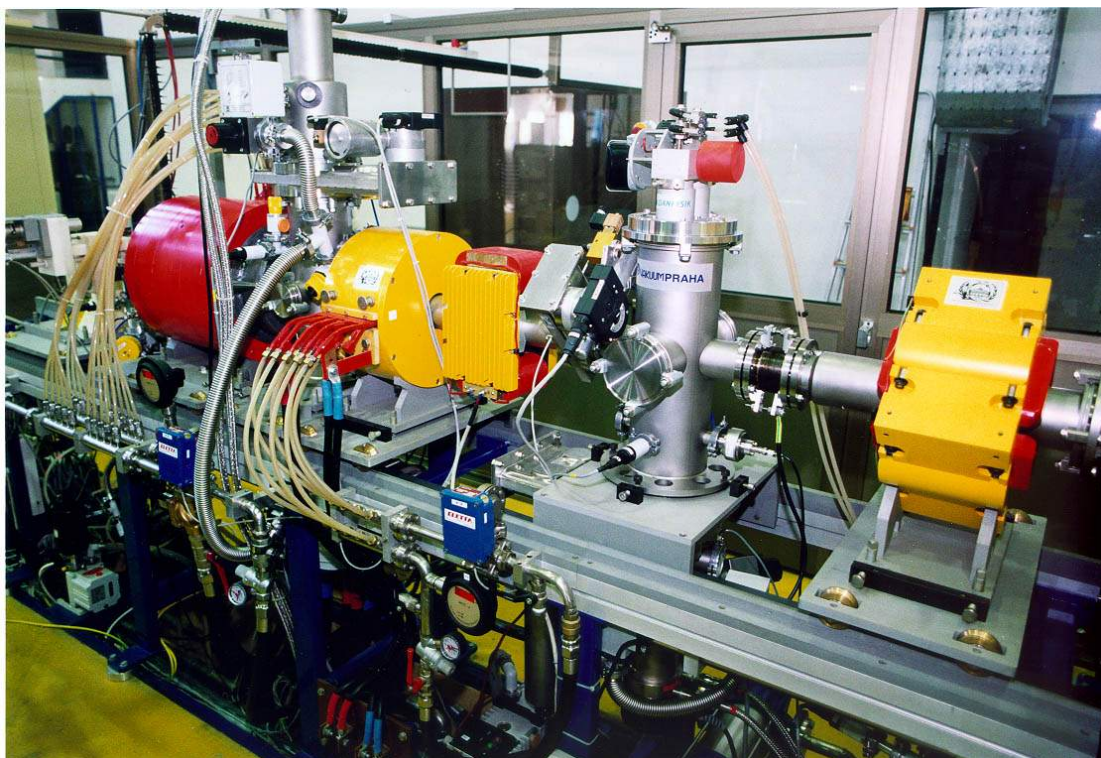
Fig. 1: mVINIS Ion Source
