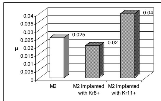
Fig. 6: Friction coefficient \mu - steel M2, F=10N .
