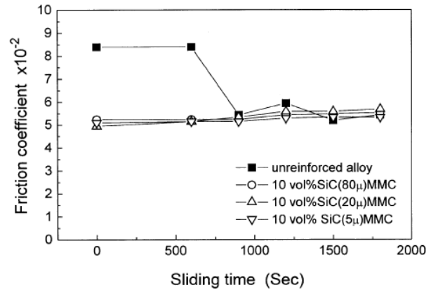
Figure 4. Friction coefficient vs sliding time for unreinforced ZA27 alloy and MMCs containing SiC particles of various sizes [10]
