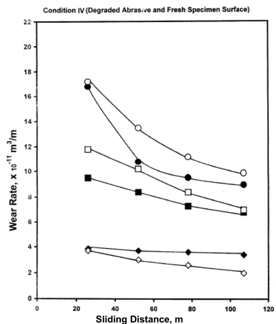
Figure 5. Wear rate of the specimens as a function of sliding distance at various applied loads in experimental condition (open symbols: composite, closed symbols: matrix alloy, ♦: 1N, ■: 3N, ▲: 5N, ●: 7 N [13])
