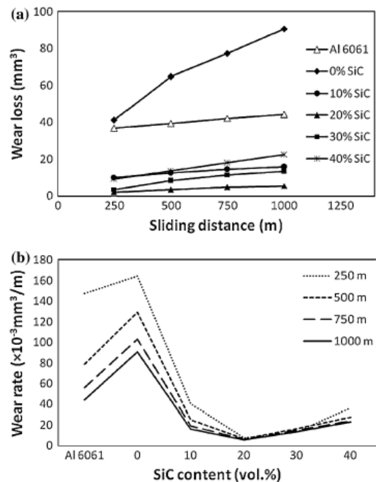
Figure 13. The variation of a wear loss with a) sliding distance and b) wear rate with SiC content for the hybrid composites containing 9 vol. % Gr particles [31]
