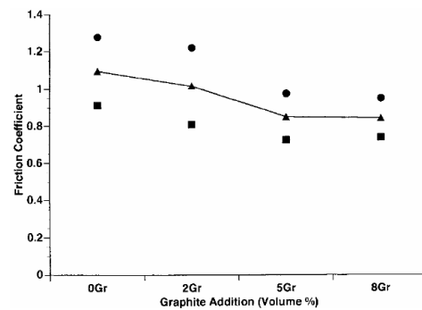
Figure 6. Variations of friction coefficient with the percentage of graphite addition [19]
