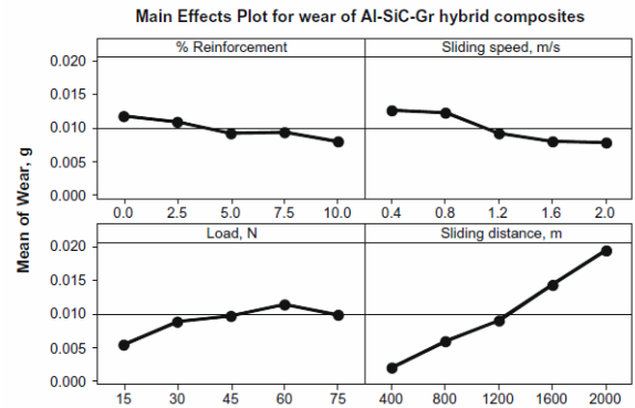
Figure 10. Main effect plot of effect of factors on wear of Al-SiC-Gr hybrid composites [23, 24, 25]
