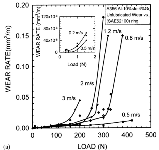
Figure 11. Wear volume vs. applied load [26]
