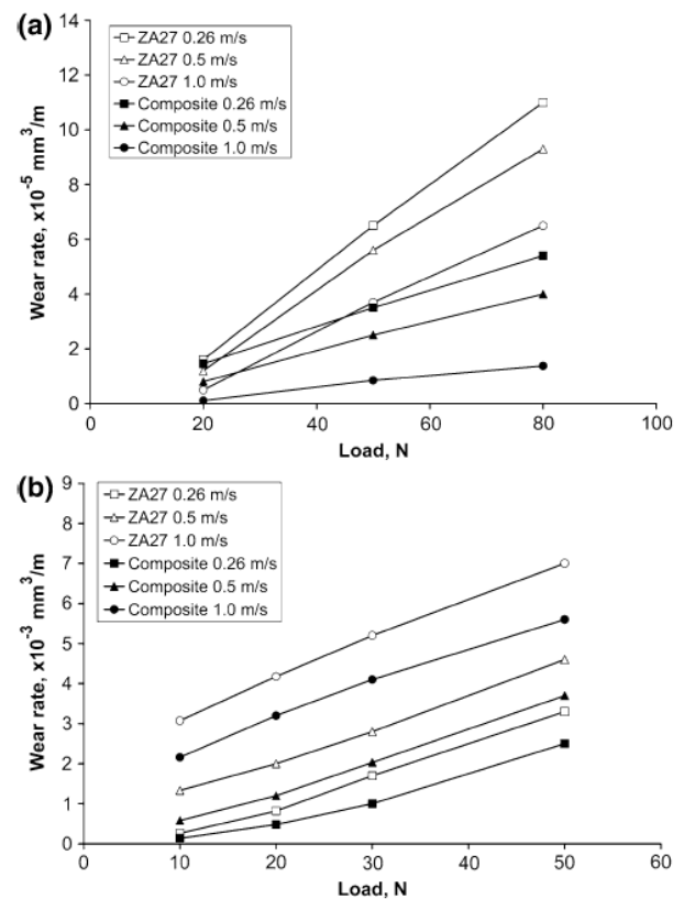
Figure 2. Wear volume vs. applied load a) Lubricated sliding, b) dry sliding [2, 4]
