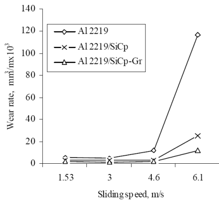
Figure 8. The wear rate variation with sliding speed for both composites and its matrix alloy [20, 21, 22]
