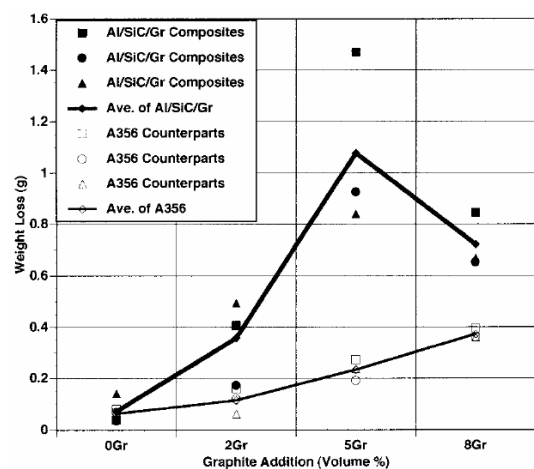
Figure 7. Weight loss of the composites and the counterparts for various graphite additions [19]
