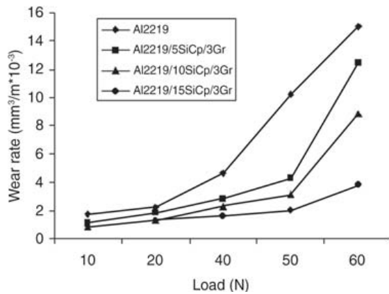
Figure 9. Variation of wear rate with applied load at a sliding speed of 3 m/s for a sliding distance of 5000 m [20, 21, 22]
