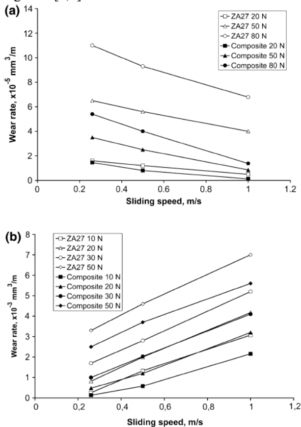
Figure 3. Wear curves of tested materials a) Lubricated sliding, b) dry sliding [2, 4]
