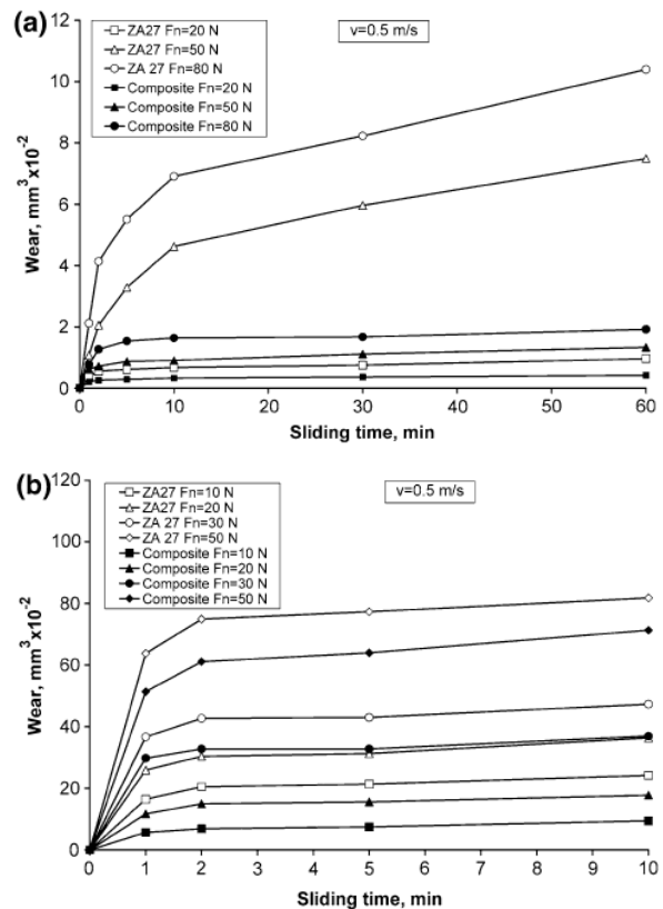
Figure 1. Wear curves of tested materials a) Lubricated sliding, b) dry sliding [2, 4]
