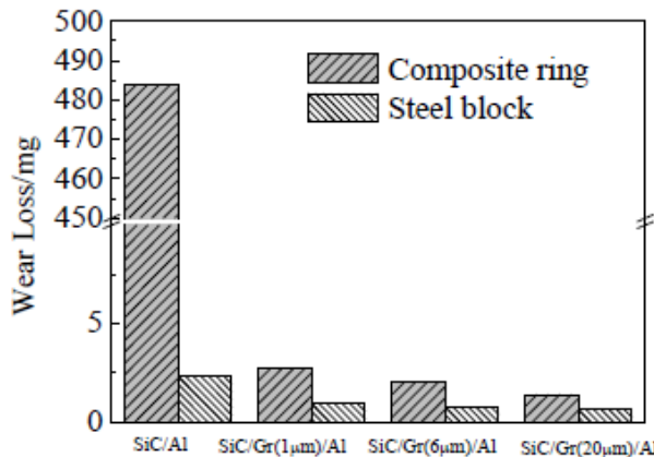
Figure 12. Wear loss of the composites and counterfaces of wear process for SiC/Al and SiC/Gr/Al [27, 28, 29]
