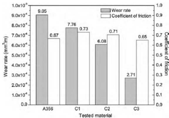
Figure 14. Wear rate and coefficient of friction values of heat treated (T6) A356 aluminium alloy, composite C1 (with 10wt% Al 2 O 3 particles), composite C2 (with 10wt% SiC particles), and composite C3 (with 10wt% SiC and 1wt% graphite particles) [32, 33]
