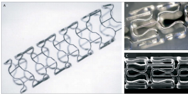
Figure 2. Bioabsorbable magnesium stent (Biotronik, Berlin, Germany) [6].
