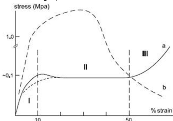
Figure 1. Stress - strain behaviour of foams.
