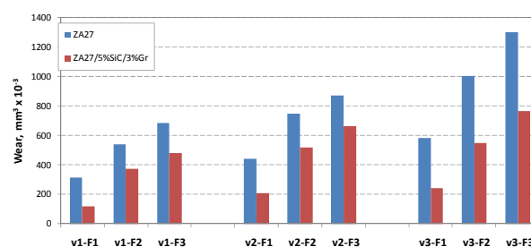
Figure 11. Comparative histograms of wear volume of ZA27 alloy and ZA27/5%SiC/3%Gr composite.
