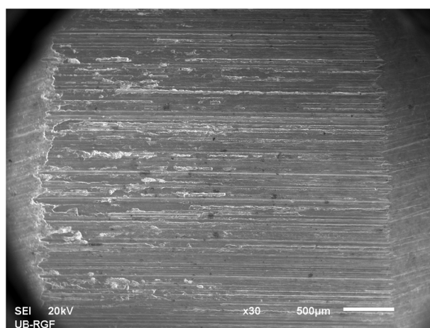
Figure 15. Appearance of the worn surface of ZA27/5%SiC/3%Gr composite photographed by SEM in dry sliding conditions ( v_1 = 0.25 m/s, F_1 = 10 N)
