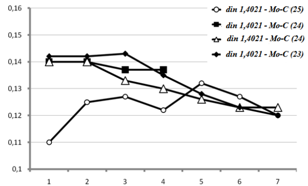
Fig. 6. Dependence of friction coefficient on loads for a friction pair Mo-C/steel DIN 1.4021 20X3MBΦ (ЭИ 415).
