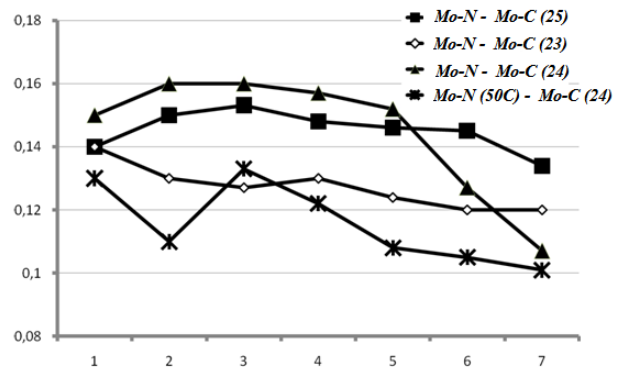
Fig. 7. Dependence of friction coefficient on a loading for a friction pair Mo-C / Avinit coating (on the basis of Mo-N).
