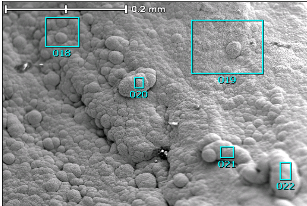
Fig. 4. A microrelief of a surface of the sample (steel DIN 1.7709 (25X2MΦ (ЭИ10))).
