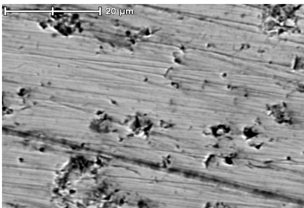
Fig. 5. A microrelief of a surface of the sample (steel DIN 1.2379 (X12Φ1)) after its polishing.
