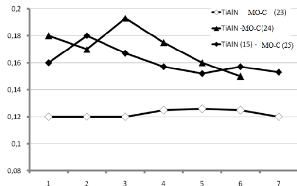
Fig. 8. Dependence of friction coefficient on a loading for a pair of a friction Mo-C / Avinit coating (on the basis of Ti-Al-N).
