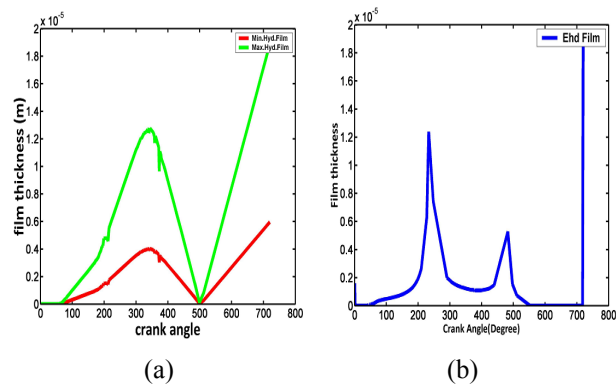
Figure 3. : For Oil A, At 500 rpm (a) Film thickness profiles (b) EHL film
