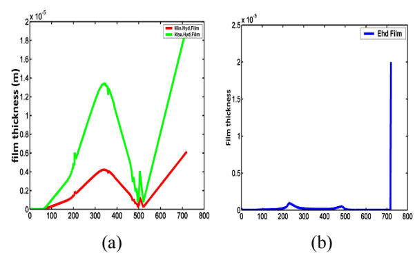
Figure 6. : For Oil B, At 500 rpm (a) Film thickness profiles (b) EHL film
