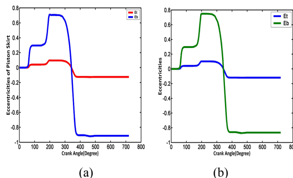
Figure 1. For Oil A , Dimensionless Eccentricities at 500 rpm in (a) Hydrodynamic regime (b) EHL Regime
