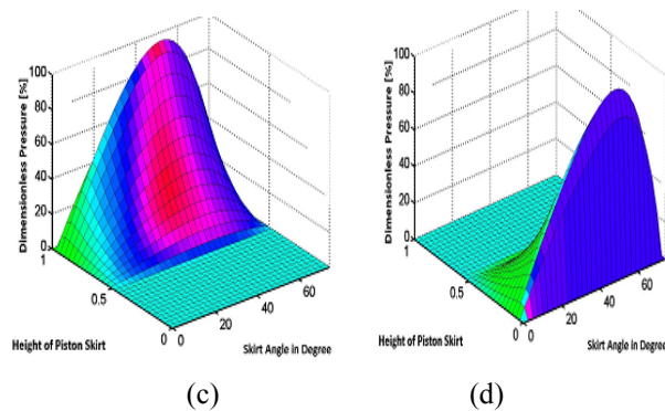
Figure 2. : For Oil A, 3-D Hydrodynamic pressure fields at 500 rpm at crank angle (a) 90 degree (b) 450 degree (c) 630 degree (d) 720 degree
