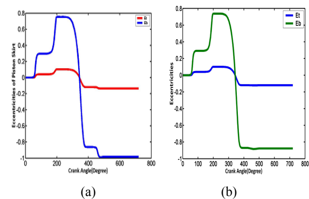
Figure 4. For Oil B, Dimensionless Eccentricities at 500 rpm in (a) Hydrodynamic regime (b) EHL Regime
