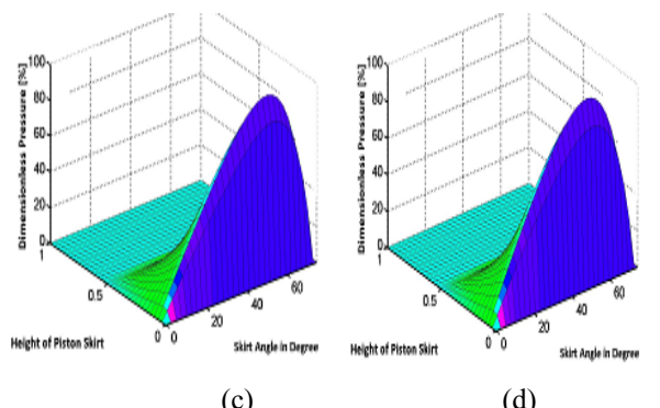
Figure 5. : For Oil B, 3-D Hydrodynamic pressure fields at 500 rpm at crank angle (a) 90 degree (b) 450 degree (c) 630 degree (d) 720 degree
