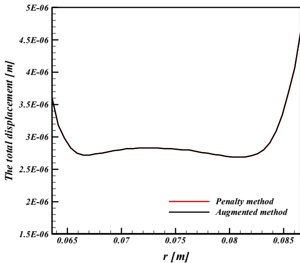
Figure 11. The variation of total displacement with disc radius (flywheel / clutch disc)
