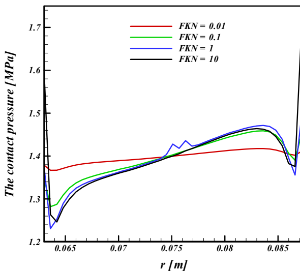
Figure 13. The variation of contact pressure with disc radius using Penalty method (flywheel / clutch disc)
