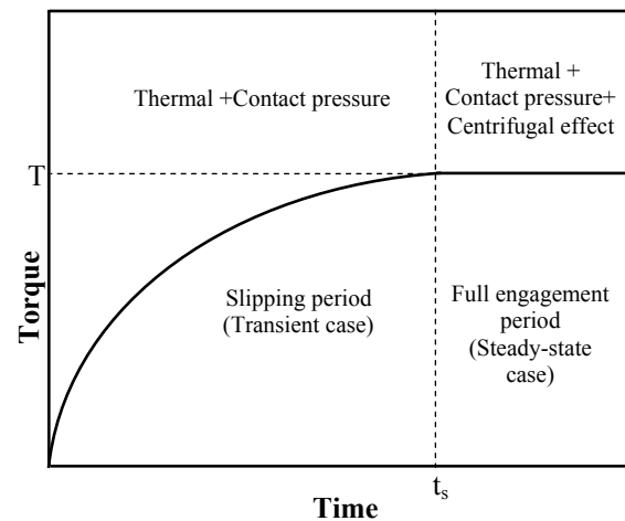
Figure 2. The load conditions during the engagement cycle of the clutch
