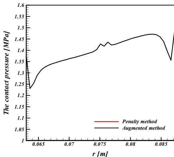
Figure 7. The variation of contact pressure with disc radius (flywheel / clutch disc)
