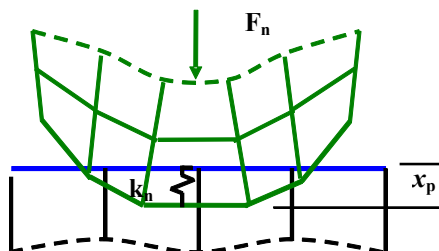
Figure 5. The contact stiffness between two contact bodies
