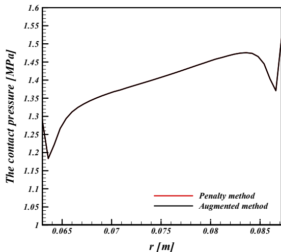
Figure 8. The variation of contact pressure with disc radius (pressure plate / clutch disc)
