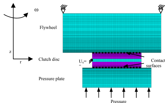
Figure 6. FE models with the boundary conditions.
