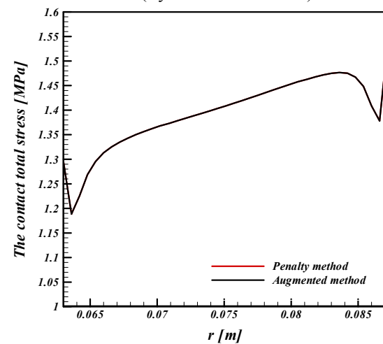
Figure 10. The variation of total contact stress with disc radius (pressure plate / clutch disc)
