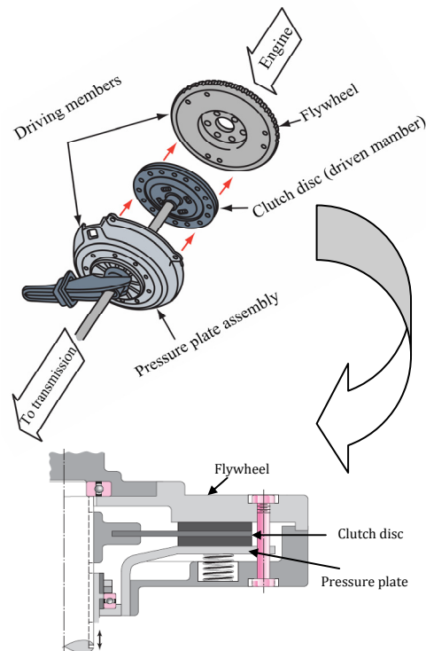
Figure 1. The main parts of clutch system
