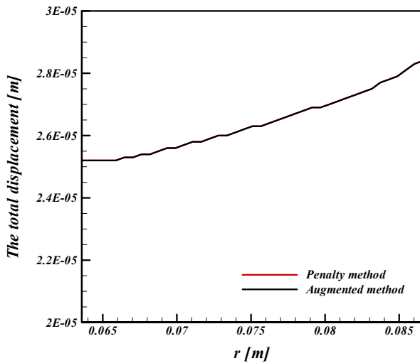
Figure 12. The variation of total displacement with disc radius (pressure plate / clutch disc)
