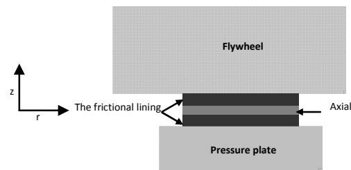
Figure 3. The Contact model for clutch system
