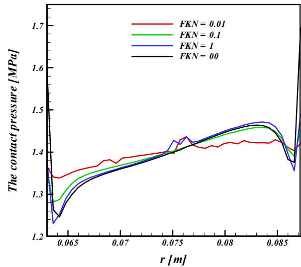
Figure 14. The variation of contact pressure with disc radius using augmented Lagrange algorithm (flywheel / clutch disc)
