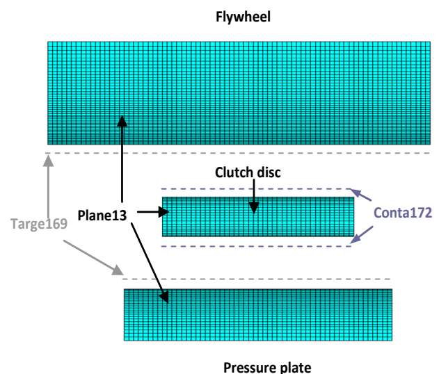
Figure 4. Schematic elements used for the friction clutch elements
