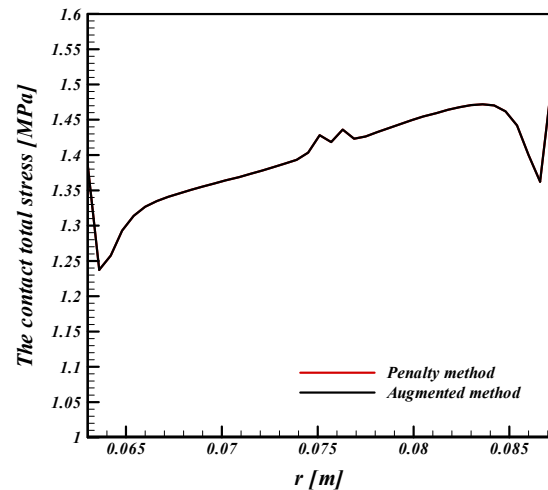
Figure 9. The variation of total contact stress with disc radius (flywheel / clutch disc)
