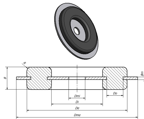
Figure 4. The basic rubber metal spring element of buffing gear
