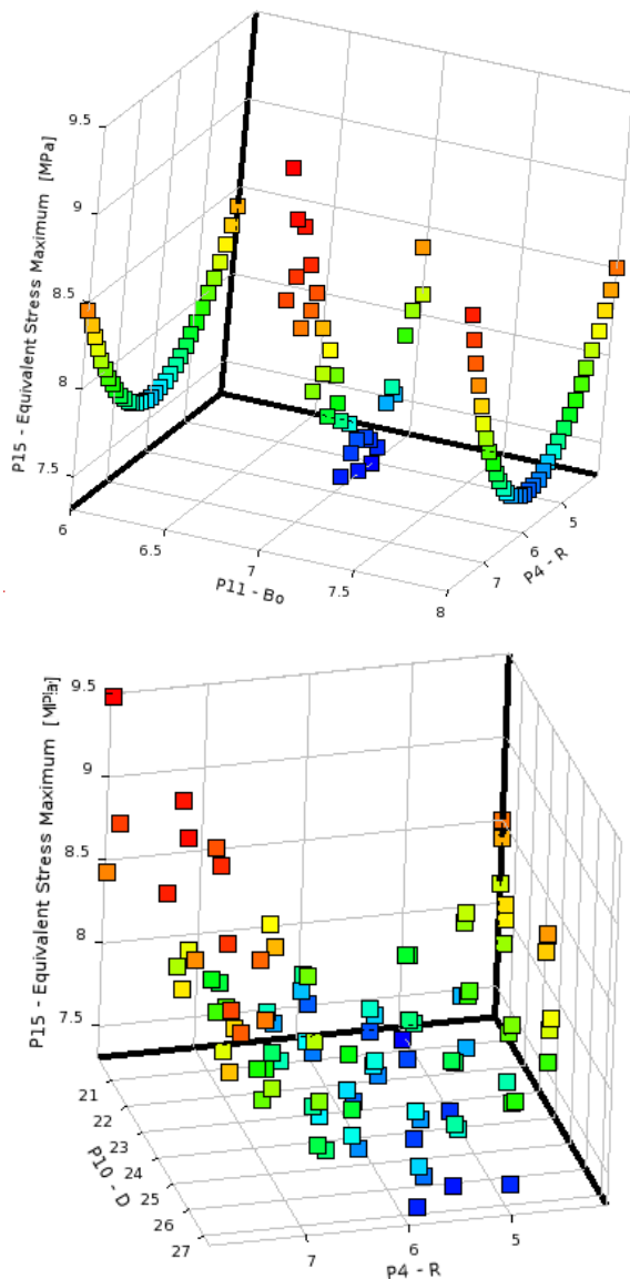
Figure 6. Functional dependence of maximal equivalent stress from the optimisation parameters
