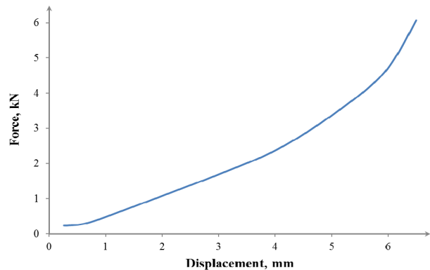
Figure 9. Experimental force – displacement data
