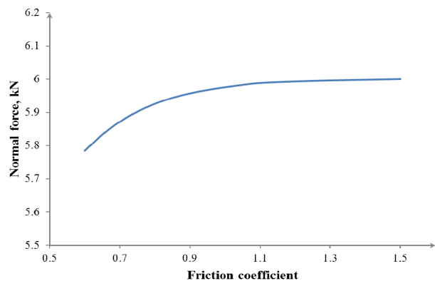
Figure 10. Functional dependence between friction coefficient and force determined by virtual experiment
