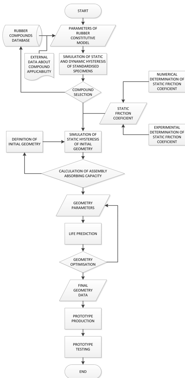
Figure 3. Procedure for development of shock absorbers with rubber-metal spring
