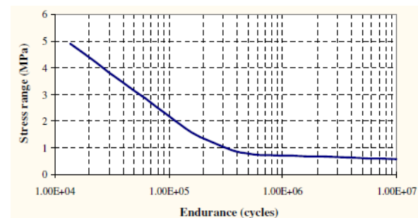
Figure 5. S-N curves of the rubber-metal element [7]
