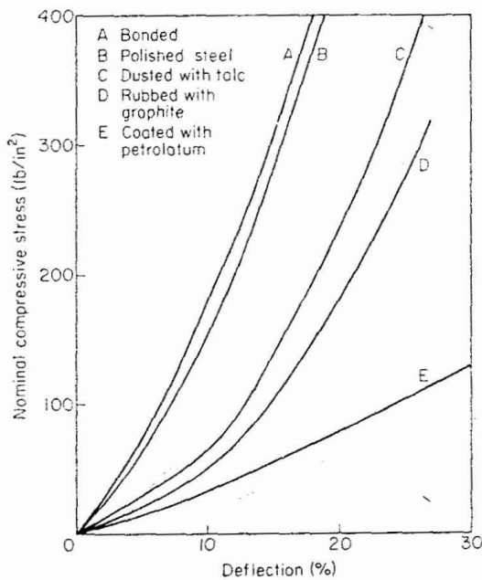
Figure 8. Effects of surface conditions on the stress/deflection curve for rubber under compression [8]
