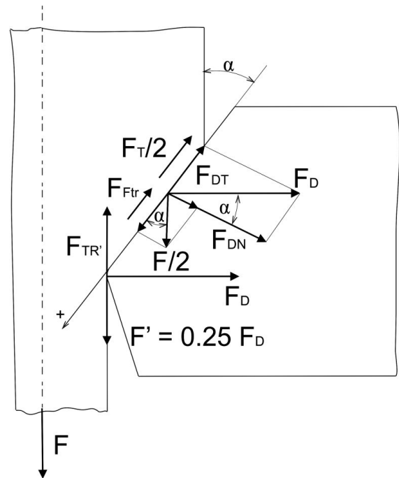
Figure 2. Force acting scheme [9]
