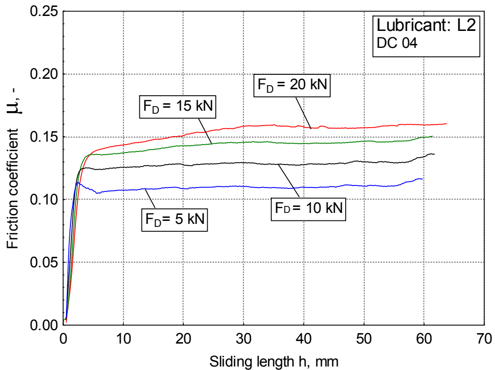
Figure 6. Friction coefficient dependencies on sliding length
