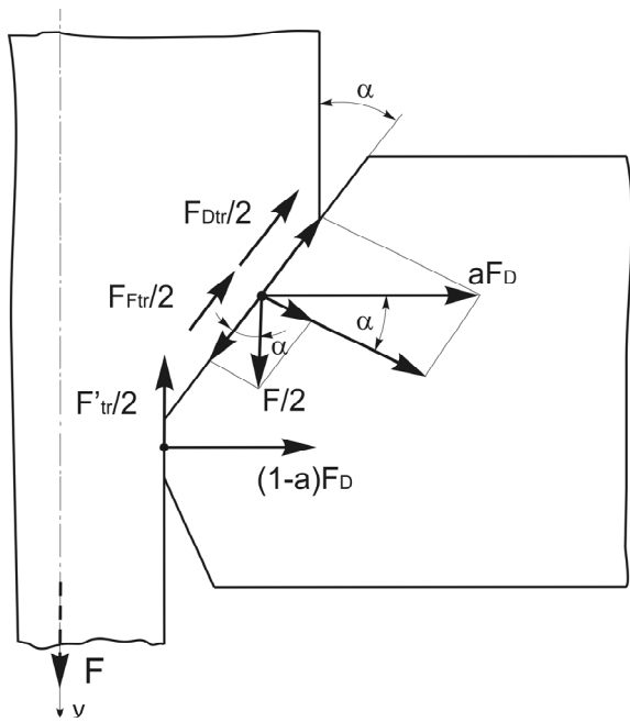
Figure 3. Modified force acting scheme
