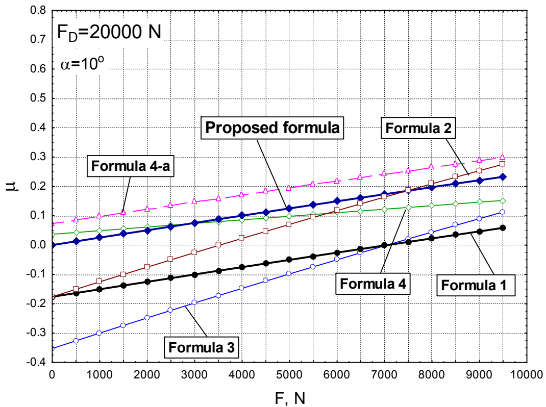
Figure 5. Friction coefficient dependencies on drawing force
