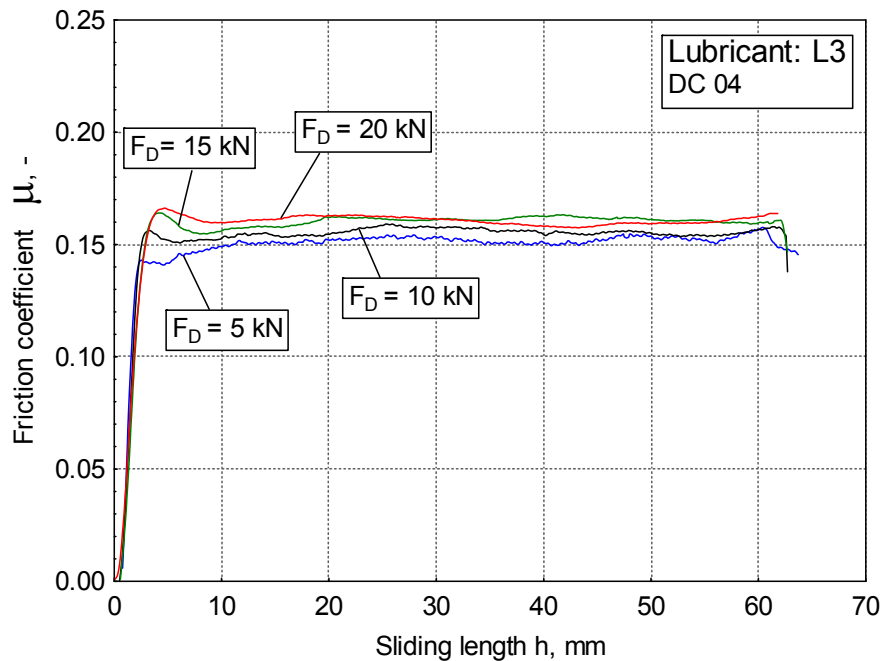
Figure 7. Friction coefficient dependencies on sliding length
