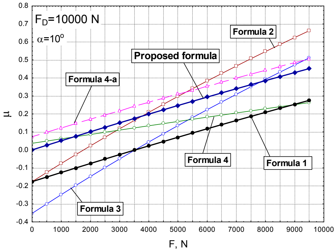
Figure 4. Friction coefficient dependencies on drawing force
