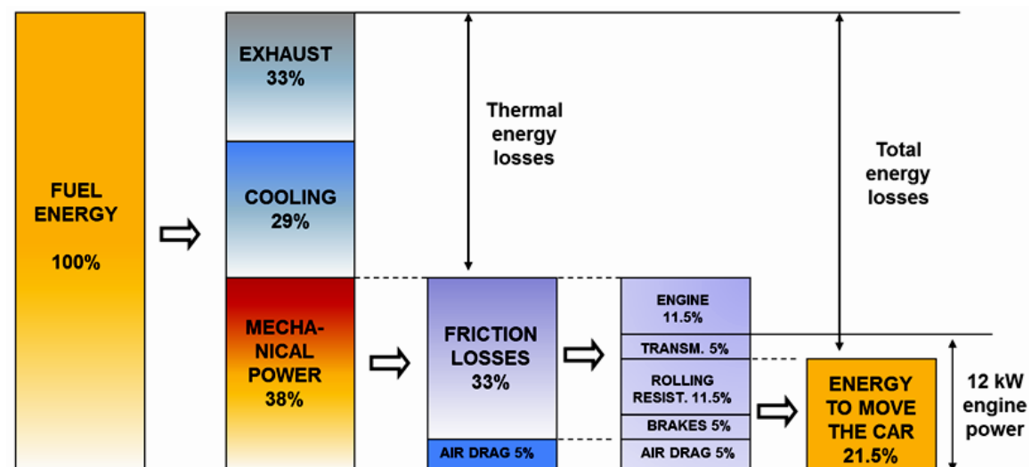
Figure 2. Breakdown of passenger car fuel energy consumption [4]
