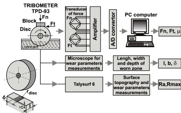
Figure 1. Measuring system for the determination of wear characteristics
