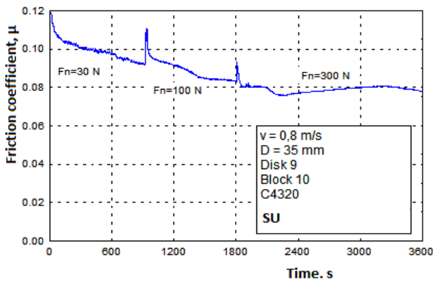
Figure 4. Change the coefficient of friction in oil samples SU
