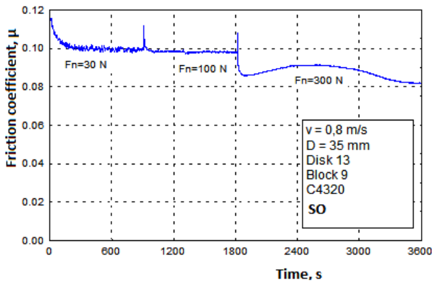
Figure 3. Change the coefficient of friction in oil samples SO
