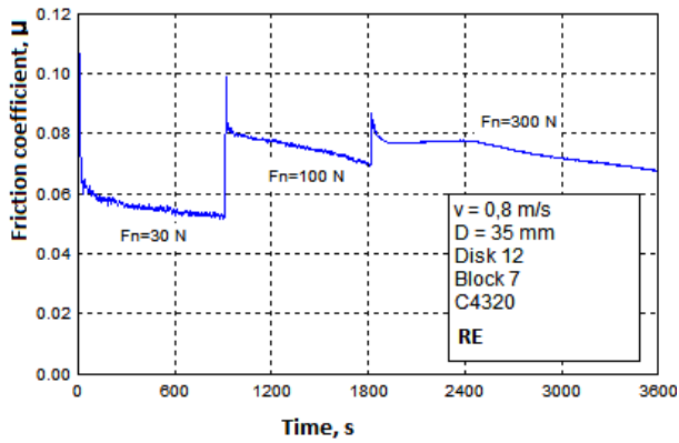
Figure 2. Change the coefficient of friction in oil samples RE
