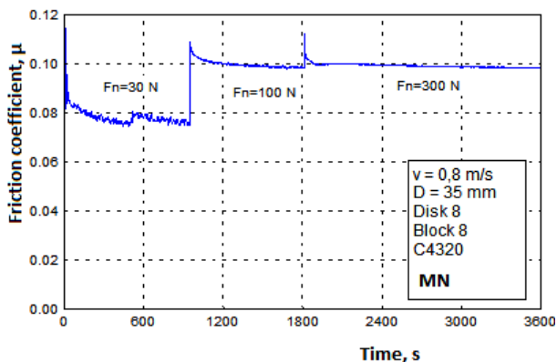
Figure 5. Change the coefficient of friction in oil samples MN
