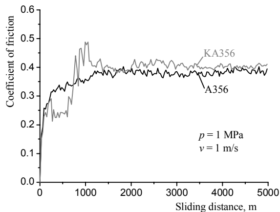
Fig. 2. Coefficient of friction vs. sliding distance for p = 1 MPa and v = 1 m/s
